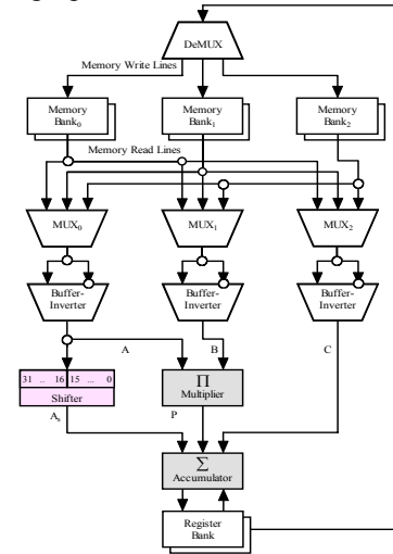
Fig. 1. Dataflow diagram
